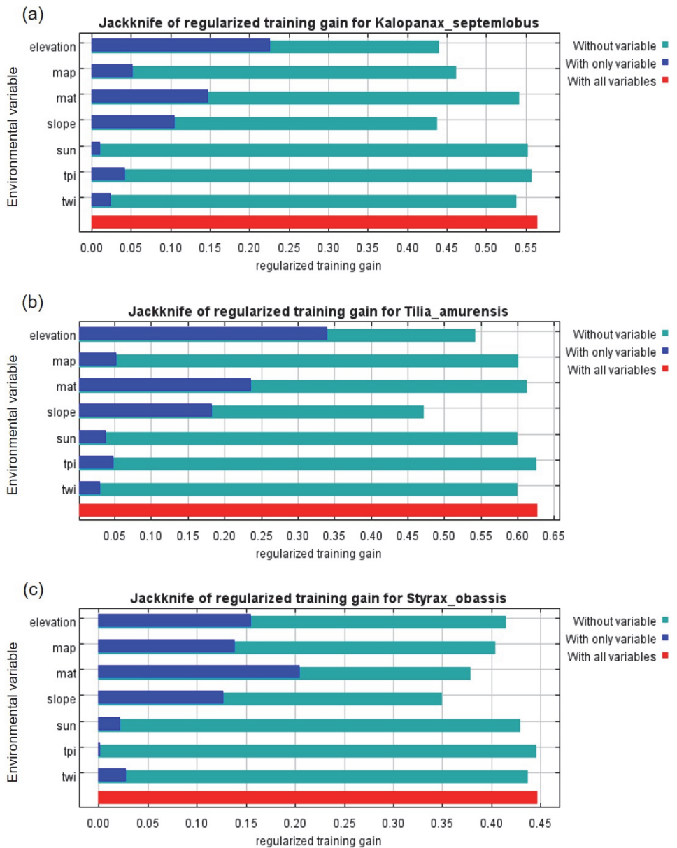
Figure 2. The relative importance (training gain) of 7 variables for (a) Kalopanax septemlobus (b) Tilia amurensis and (c) Styrax obassis . Abbreviations: map, mean annual precipitation; mat, mean annual temperature; sun, solar radiation; tpi, topographic position index; twi, topographic wetness index.
